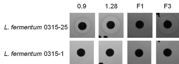
Fig. 2 Extracted antibacterial activity from DDGS does not inhibit growth of a virginiamycin resistant strain of Lactobacillus fermentum . The following samples (10 μl) were applied to a paper disc on agar plates inoculated with either L. fermentum 0315-25 (top row) or L. fermentum 0315-1 (bottom row): 0.9 μg/ml virginiamycin (0.9); 1.28 μg/ml virginiamycin (1.28); extract of DDGS from control fermentor (F1); extract of DDGS from fermentor dosed with 20 ppm virginiamycin product (F3). Minimum inhibitory concentrations for virginiamycin of L. fermentum 0315-25 and L. fermentum 0315-1 are ≤2 μg/ml and >16 μg/ml, respectively
